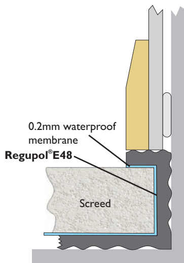
Perimeter Detail
