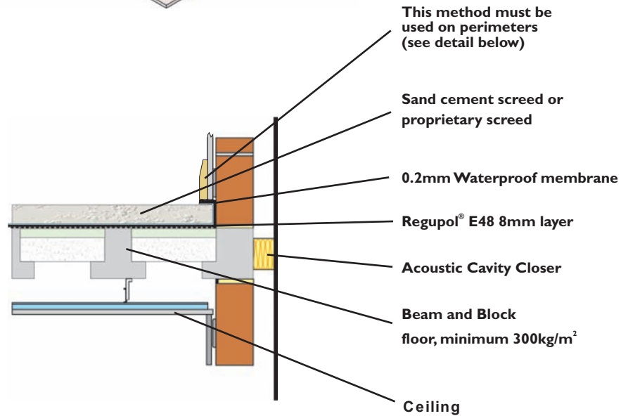
Joint Detail
