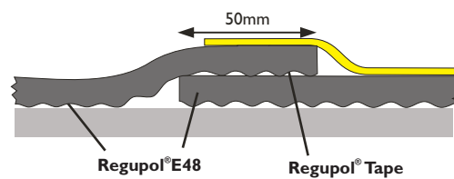
Joint Detail
